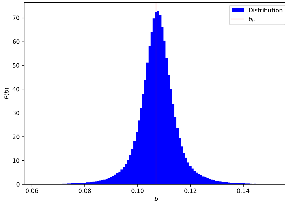
Figure 1: Probability distribution P(b) .
