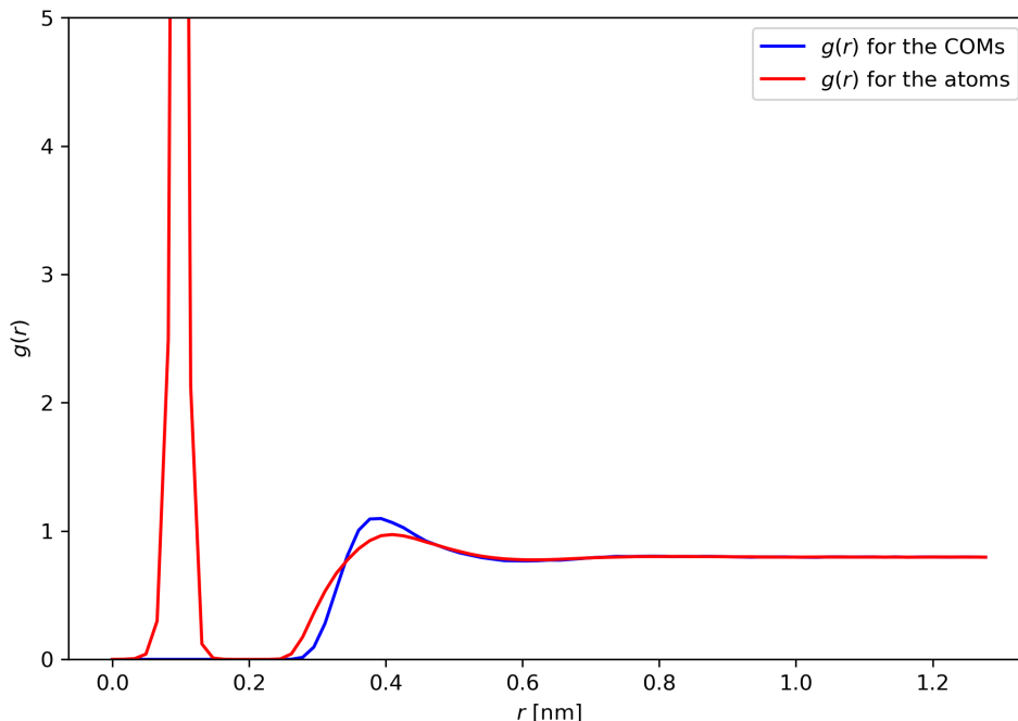
Figure 4: Radial distribution functions.
